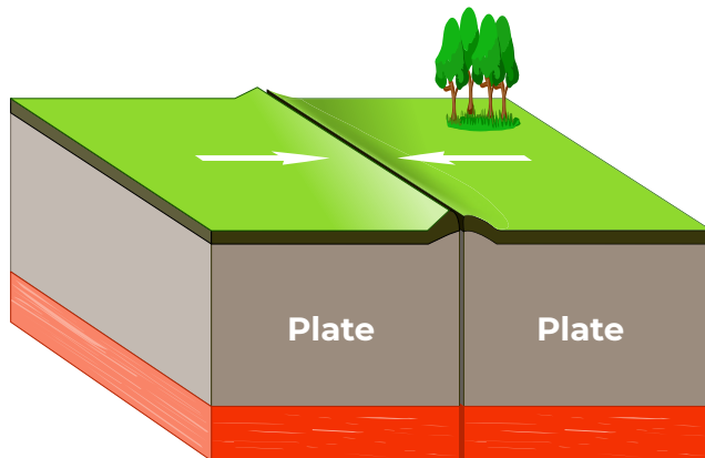
Convergent Plates Collide
