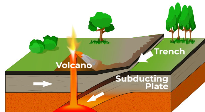
Subduction Plates Subduct
